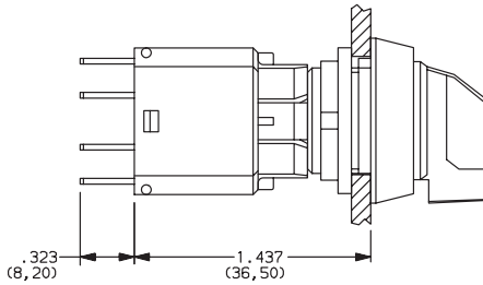
Contact Block with Momentary and Latching Selector Switch
